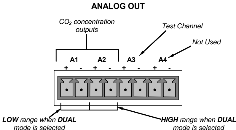
Figure 4-6: Analog Output Connector Pin Out
